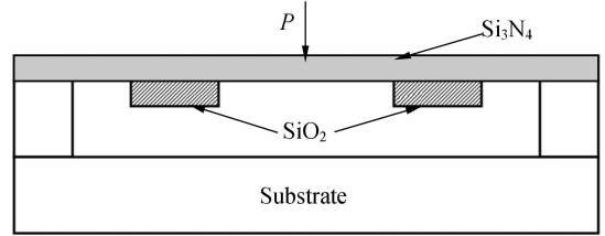
Fig. 1 Cross-section of a capacitive pressure sensor with composite diaphragm structure
