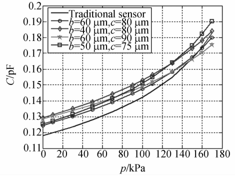
Fig. 9 Relationship between pressure and capacitance with different dimensions of the \text{SiO}_2 diaphragm ( t_{\text{SiO}_2}=0.5\ \mu\text{m} )
