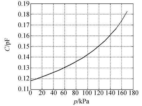
Fig. 3 Relationship between pressure and capacitance of a traditional capacitive pressure sensor
